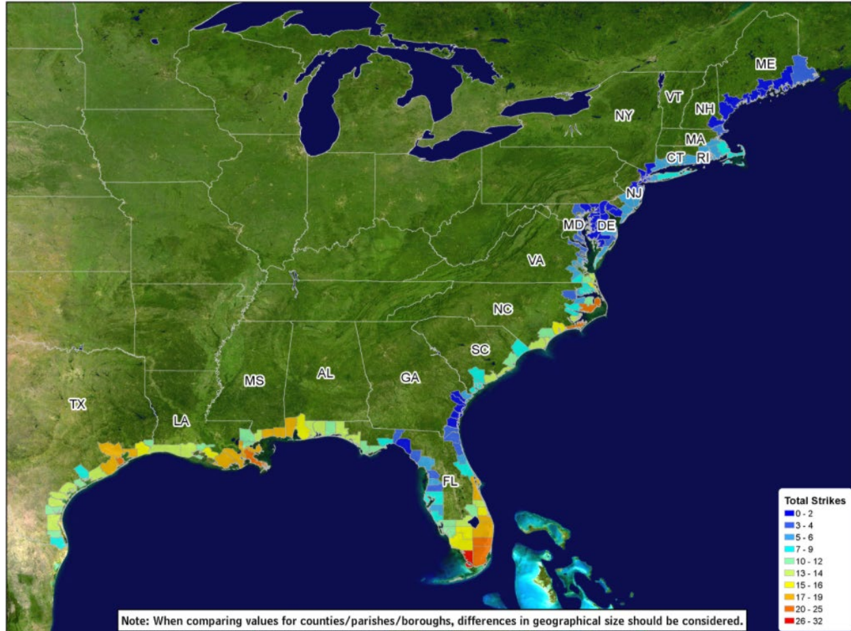
Figure 4. East Coast Hurricane Strikes 1900-2010 (NOAA, ND,e)
