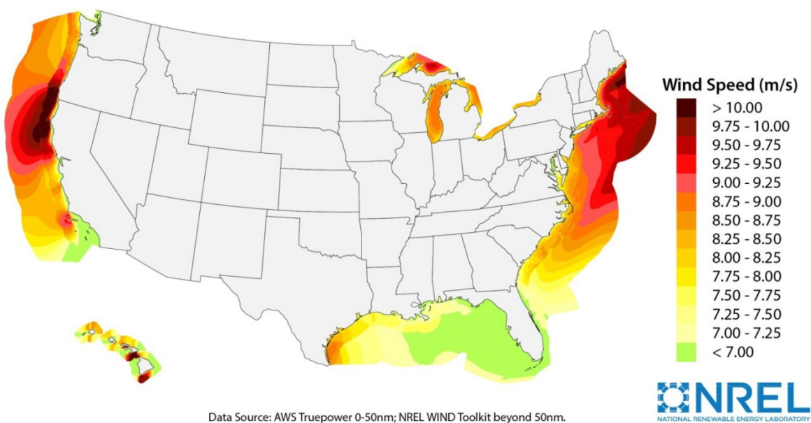
Figure 4: Offshore Wind Speeds in Coastal Areas
