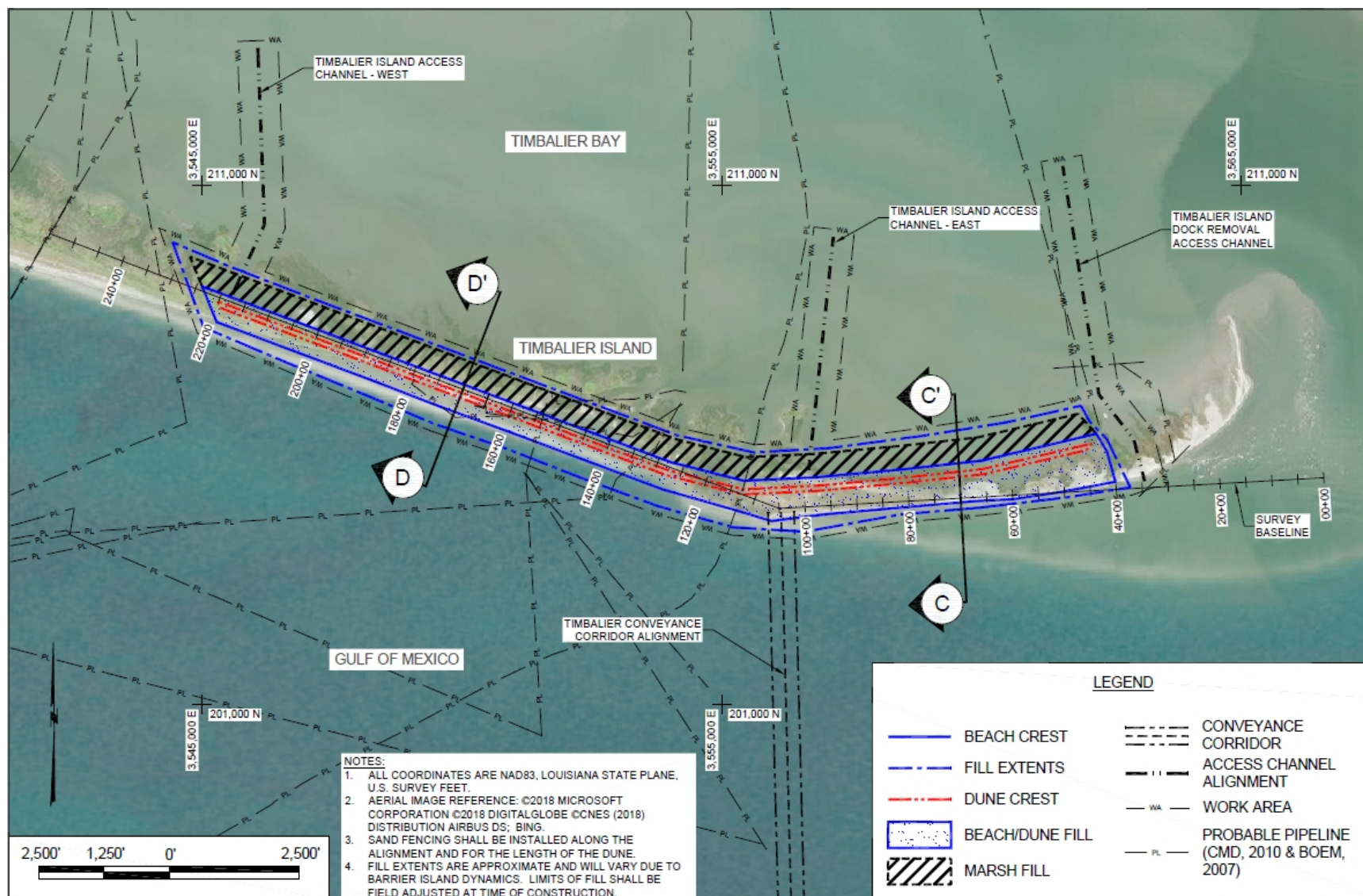
Figure 2-3. Timbalier Island Restoration Template – Plan View
